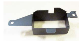
Front Log Plate (used with logs only – see Media Installation)
