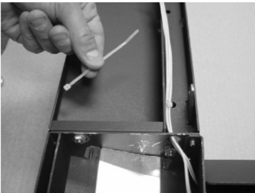
Figure 5: Lock-tie
