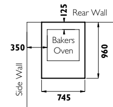
Clearances & minimum hearth requirements Door Aperture 245 x 345mm
