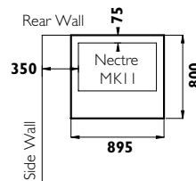
Clearances & minimum hearth requirements
