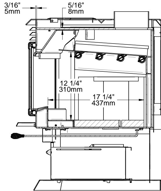
SECTION C-C
